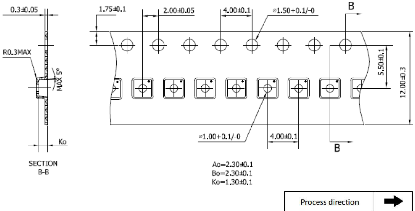
Figure 18 Tape and reel dimension in mm
