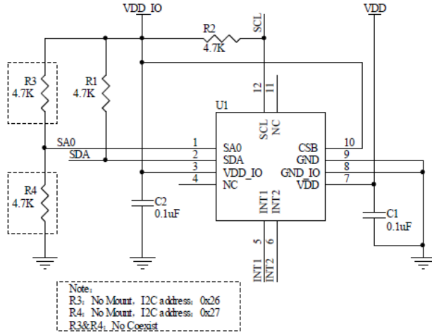
Figure 13 da618G I2C electrical connect
