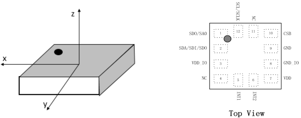
Figure 2 Pin description
