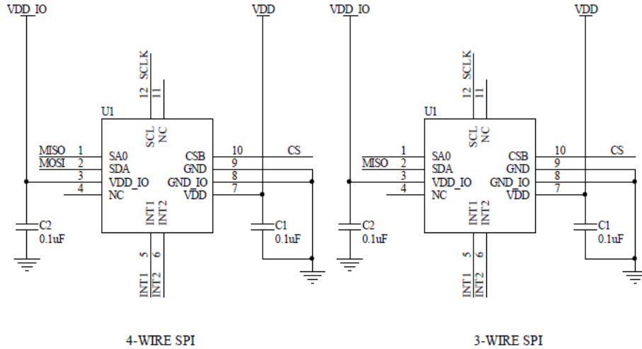
Figure 14 da618G SPI electrical connect
