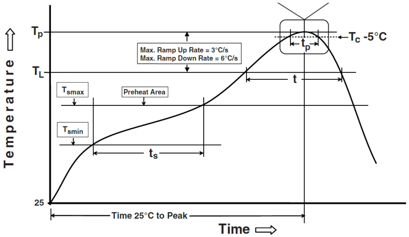
Figure 17 Soldering profile
