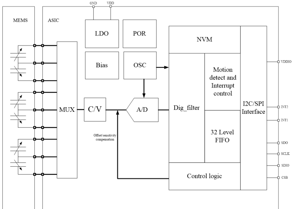
Figure 1 Block Diagram
